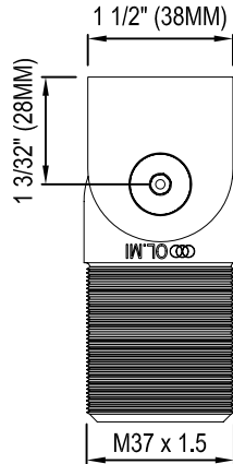
PLAN VIEW
