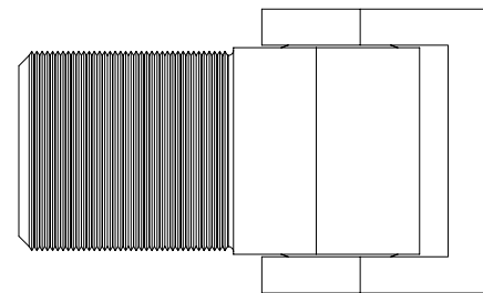
RIGHT ELEVATION VIEW
